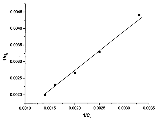
Figure 3. Langmuir plot ( 1/q_e vs. 1/C_e ). Conditions are electrolyte pH: 7; electrolyte temperature: 303 K, and current density: 0.25 A/dm 2 .
